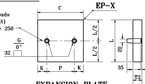
EXPANSION PLATE
