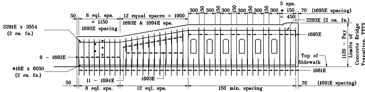
ELEVATION SHOWING REINFORCING STEEL
