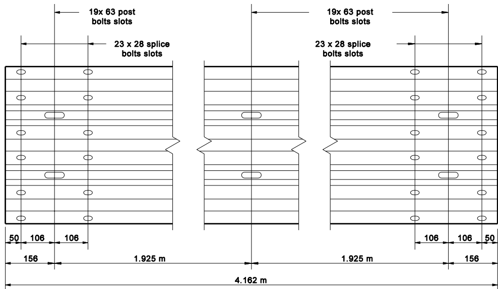
THRIE BEAM ELEVATION
