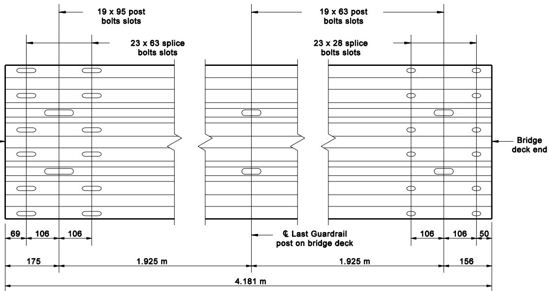
THRIE BEAM EXPANSION ELEMENT ELEVATION
