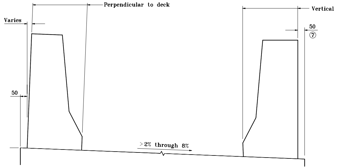
Superelevated Section
