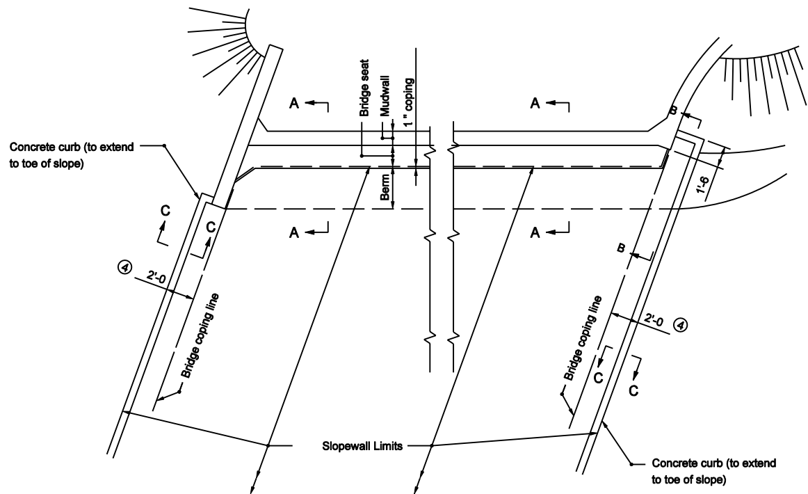
STRAIGHT WINGS
