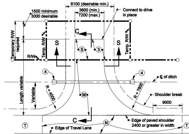
PLAN VIEW (PAVED SHOULDER 2400 OR GREATER IN WIDTH)
