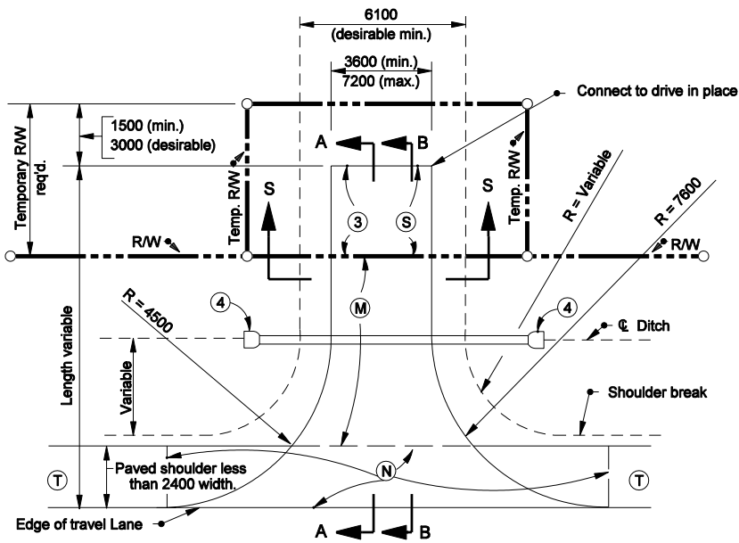
PLAN VIEW (PAVED SHOULDER LESS THAN 2400 IN WIDTH OR UNPAVED SHOULDER)
