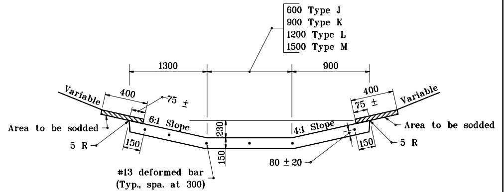
ELEVATION VIEW
