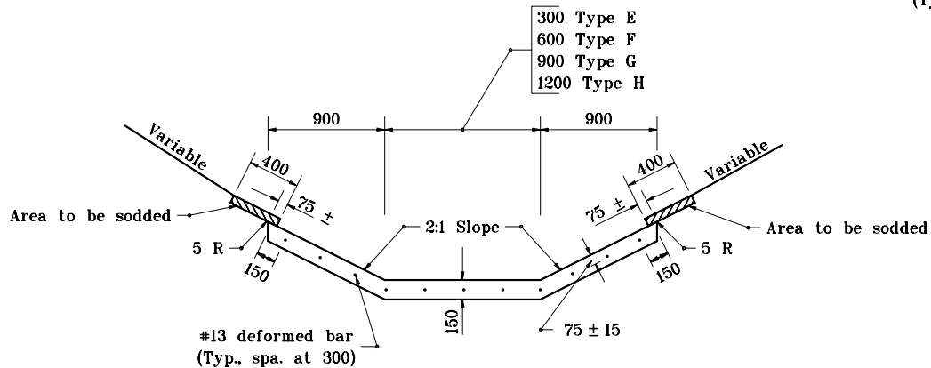
ELEVATION VIEW
