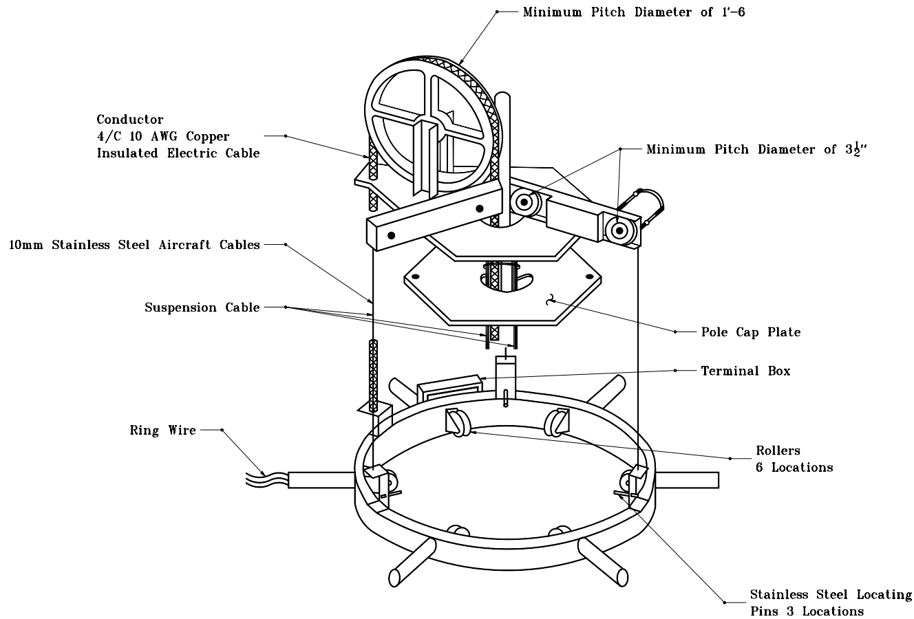
RING ASSEMBLY
