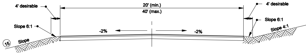
SECTION P-P - CLASS IV DRIVES
