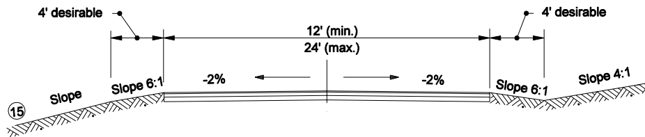
SECTION S-S - CLASS II DRIVES
