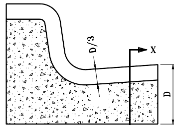
COMBINED CURB & GUTTER
