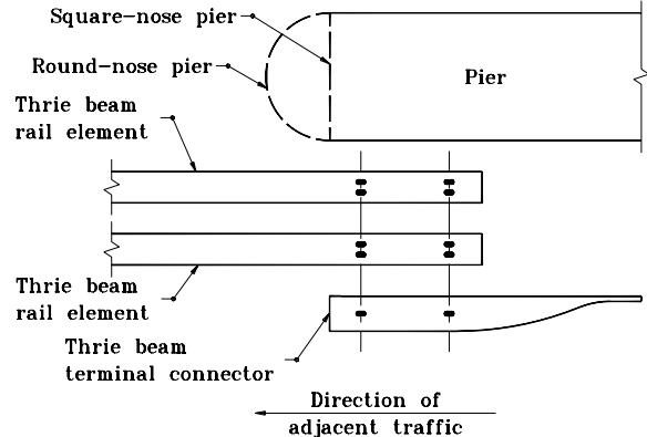
LAP DETAIL AT PIER CONNECTION
