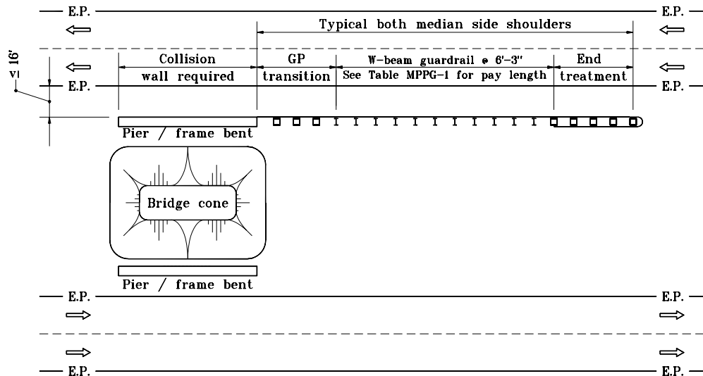
MULTI-LANE DIVIDED WITH TANDEM OVERHEAD STRUCTURE AND MEDIAN SIDE PIER TO E.P. ≤ 16'
