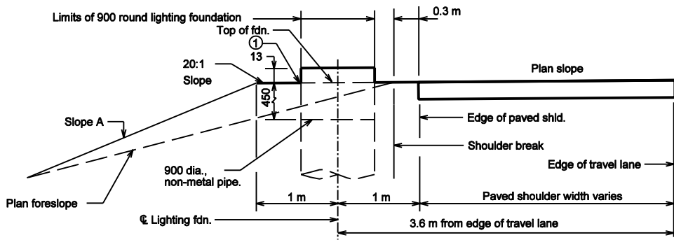
ELEVATION, 4:1 OR 3:1 SLOPE
