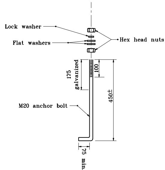
ANCHOR BOLT FOR A, M, AND P-1 FOUNDATIONS
