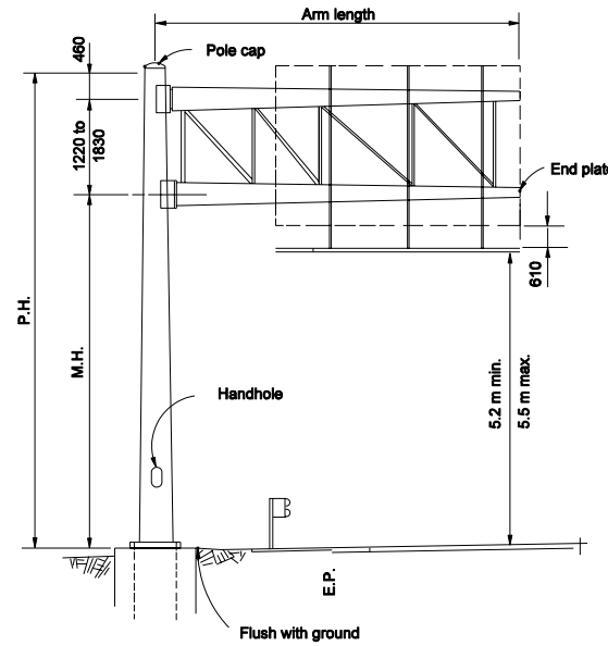
CANTILEVER (DOUBLE MASTARM)
