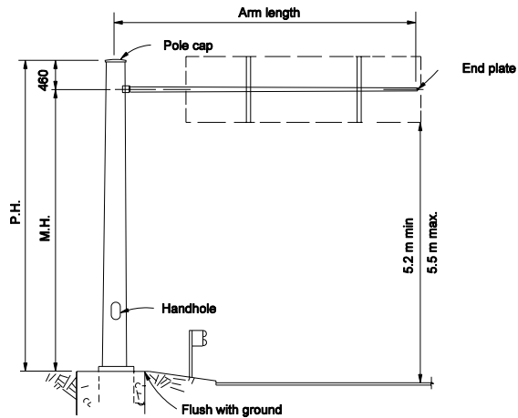
CANTILEVER (SINGLE MASTARM)
