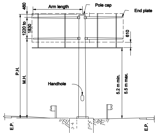
OVERHEAD BALANCED CANTILEVERS
