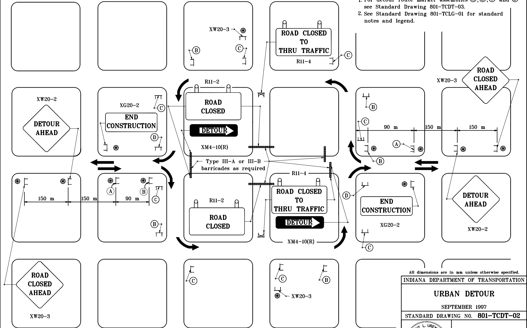
TYPICAL APPLICATIONS OF TRAFFIC DEVICES FOR AN URBAN DETOUR
