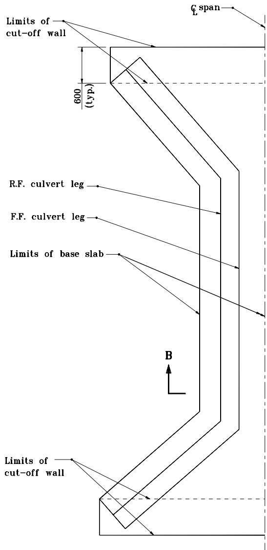
PLAN - WITH WINGWALLS
