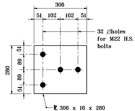
PLATE WASHER PWW
