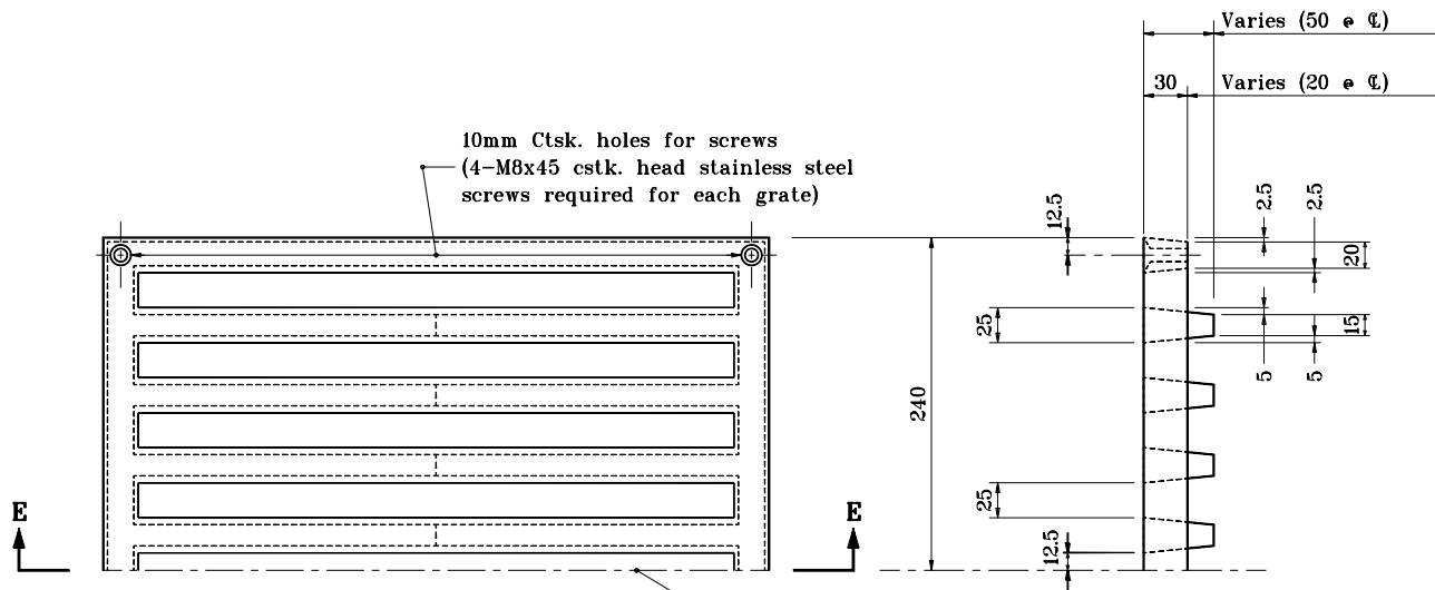
HALF PLAN
