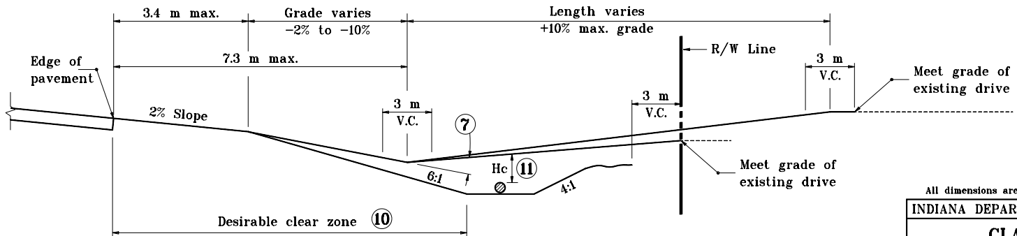
TYPICAL PROFILE GRADE IN CUT
