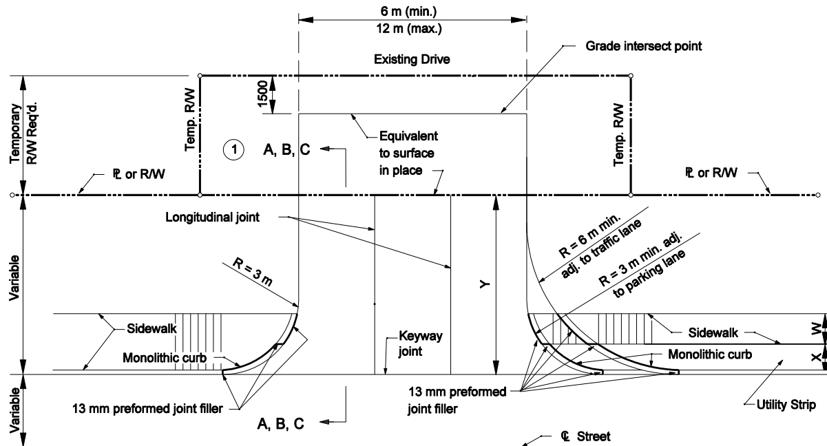
PLAN VIEW - CLASS III DRIVE
