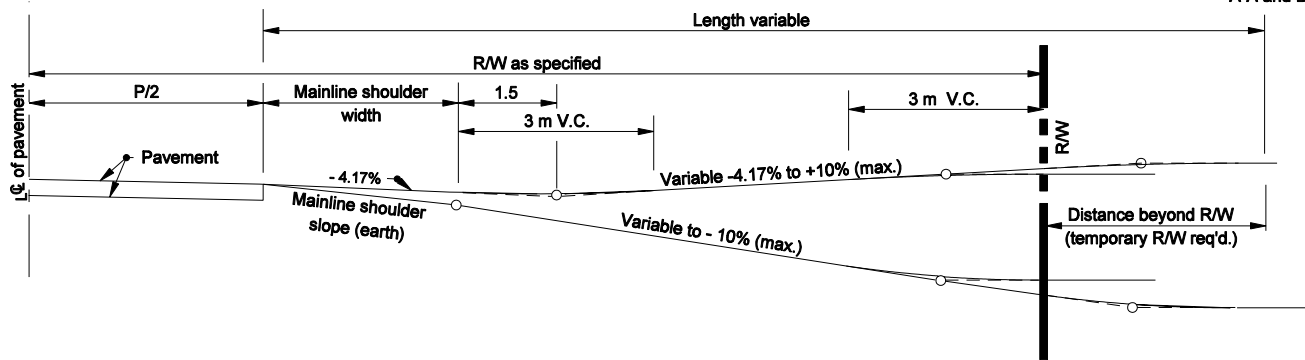
SECTION B-B APPROACH GRADE FOR CUT OR FILL TO BE USED WITH EARTH SHOULDERS
