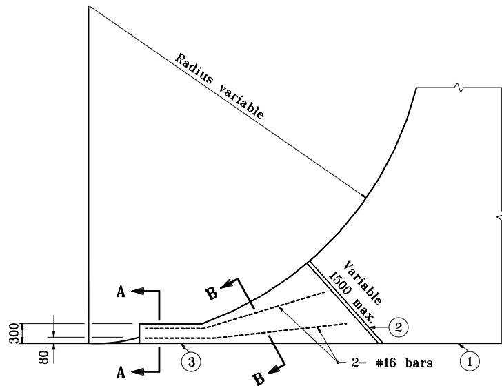
EAR CONSTRUCTION TYPE "A"
