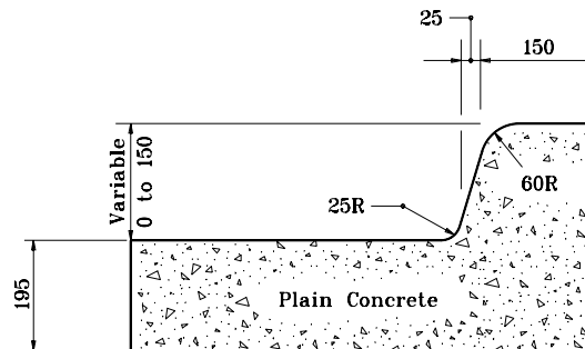
MONOLITHIC CURB
