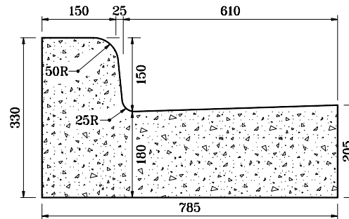
COMBINED CONCRETE CURB AND GUTTER (BARRIER)
