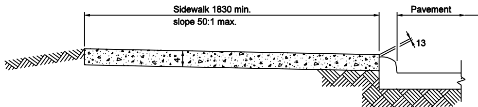
SECTION THROUGH SIDEWALK ADJACENT TO CURB
