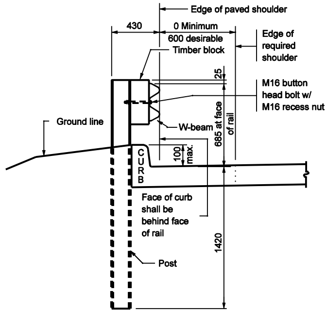
TYPICAL W-BEAM INSTALLATION AT CURB
