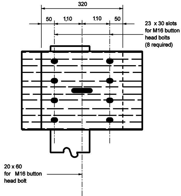
STEEL W-BEAM SPLICE DETAIL
