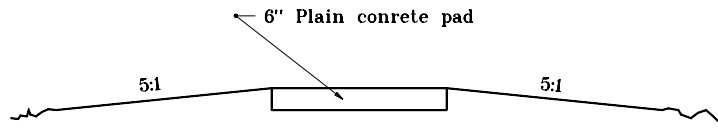
SECTION B-B
