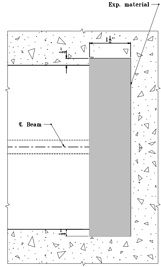
SECTION C-C
