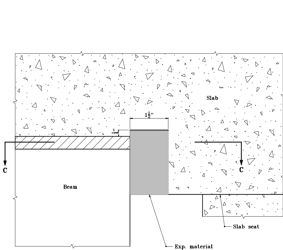
SECTION THROUGH BEAM FLANGE AND SLAB
