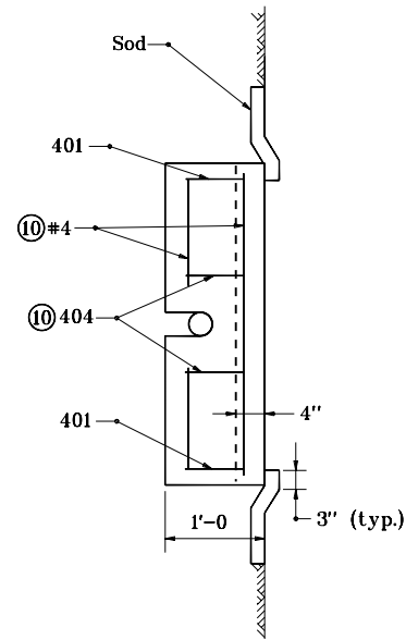
SECTION C-C
