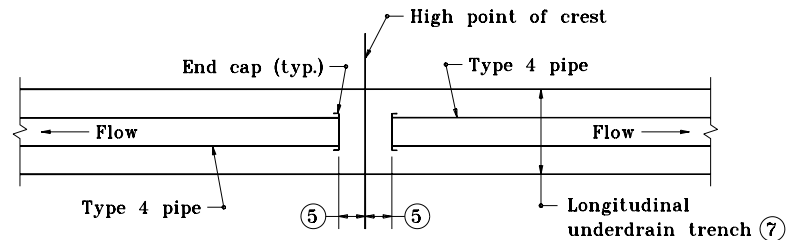
PLAN-INSTALLATION AT CREST
