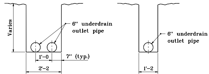
TWIN OUTLET DETAIL
