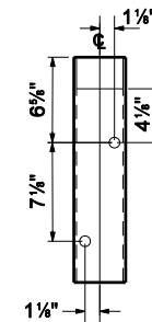
BACK VIEW
