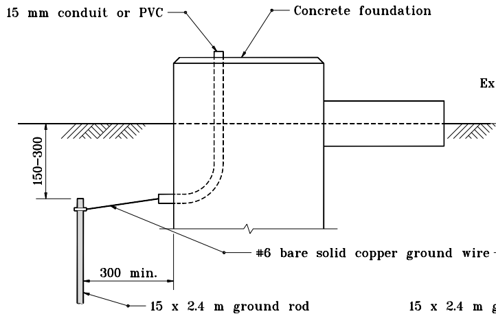
TYPICAL DETAIL GROUND ROD IN EARTH
