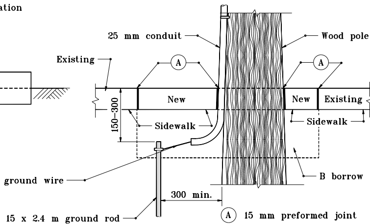
TYPICAL DETAIL GROUND ROD IN SIDEWALK
