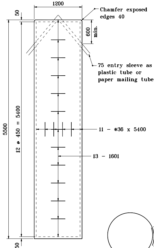
ELEVATION FOUNDATION TYPE I
