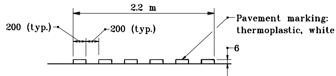
SECTION F-F
