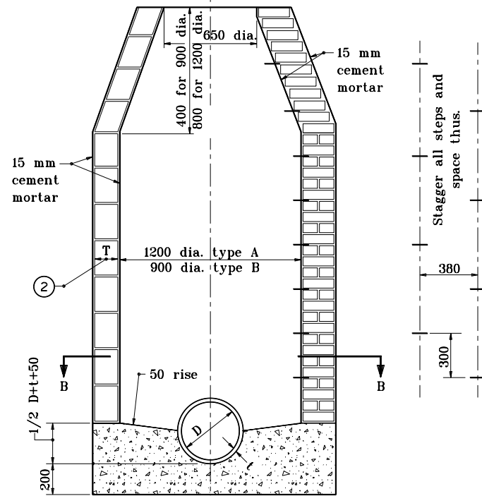
SECTION A-A TYPE A Dia. = 1200 TYPE B Dia. = 900
