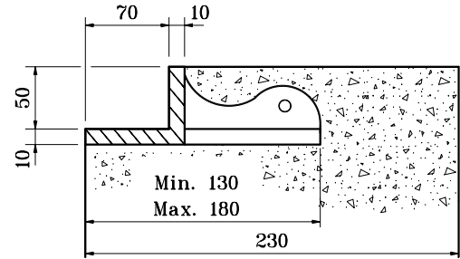
DETAIL OF ANCHOR
