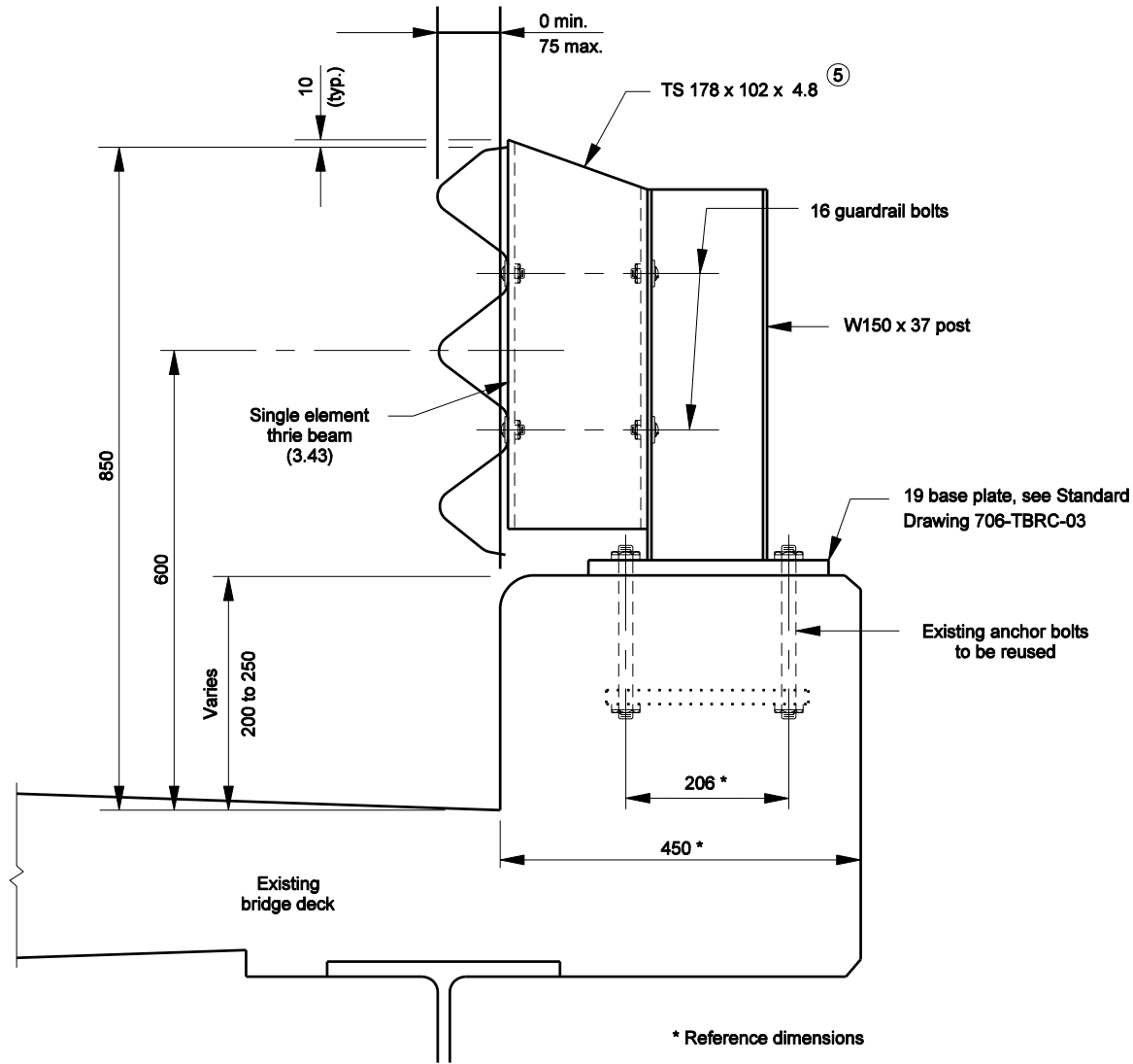
SECTION A-A CURB MOUNTED
