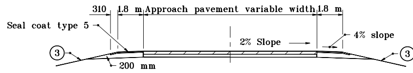
MINIMUM PAVEMENT SECTION A-A (FOR UP THROUGH 50 TRUCKS PER DAY)
