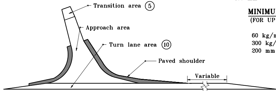
PAY LIMITS FOR BITUMINOUS MIXTURE FOR APPROACHES
