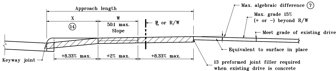
SECTION C-C
