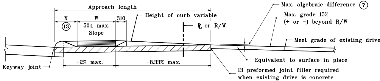
SECTION B-B
