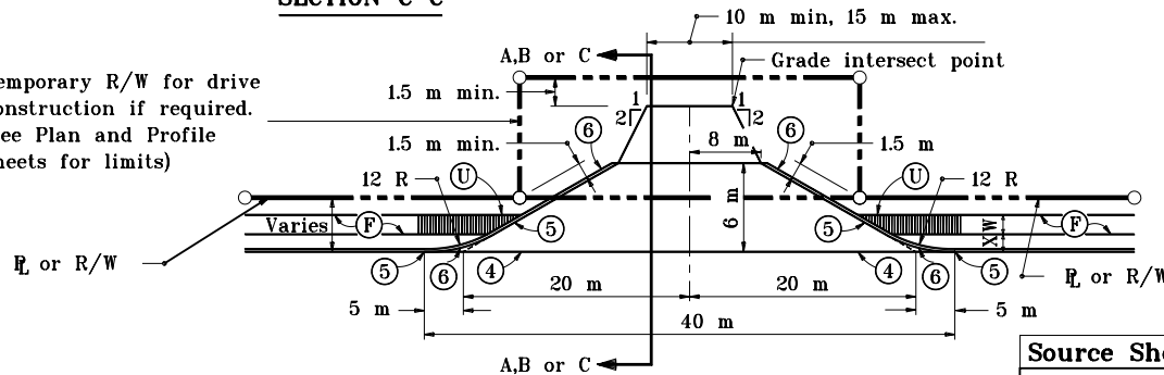
SECTION C-C
