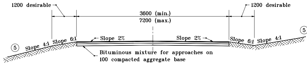
CROSS SECTION
