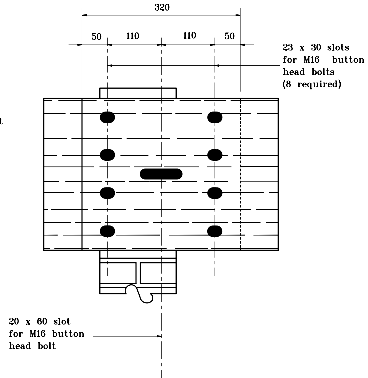
STEEL W-BEAM SPLICE DETAIL
