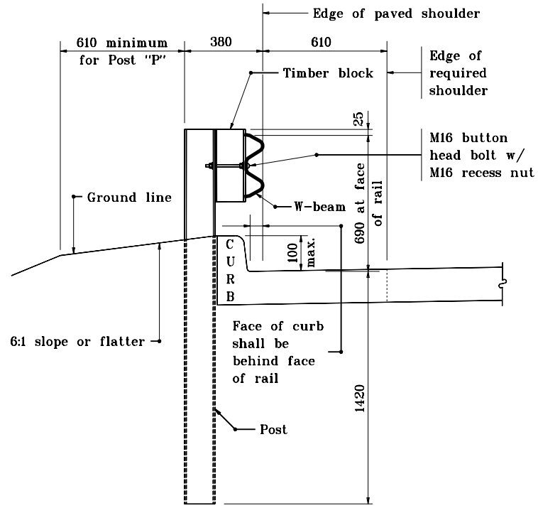
TYPICAL W-BEAM INSTALLATION AT CURB
