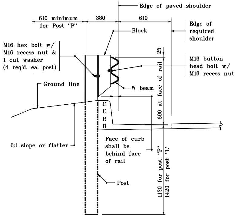
TYPICAL W-BEAM INSTALLATION • CURB
