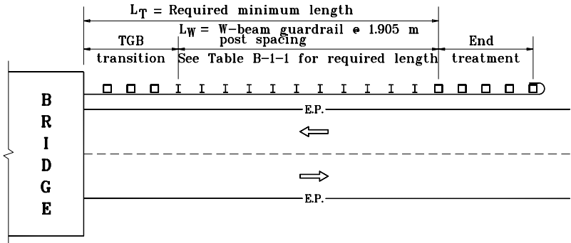
Two-Lane Two-Way Bridge Approach Guardrail Typical All Four Corners
