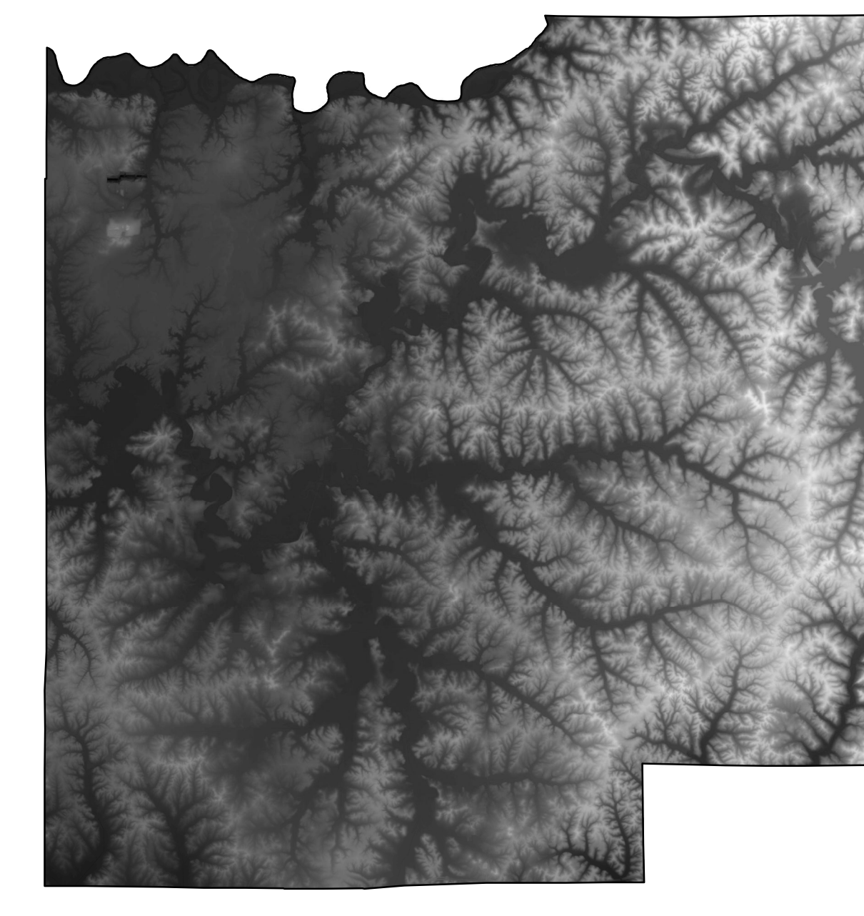
Digital Elevation Model of Dubois County, Indiana
