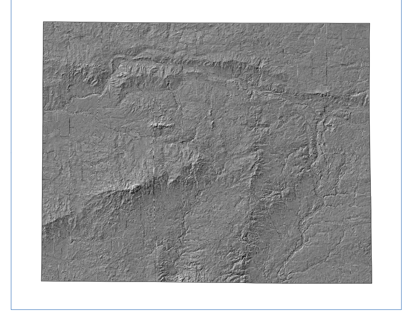
Hillshade Map of Benton County, Indiana
