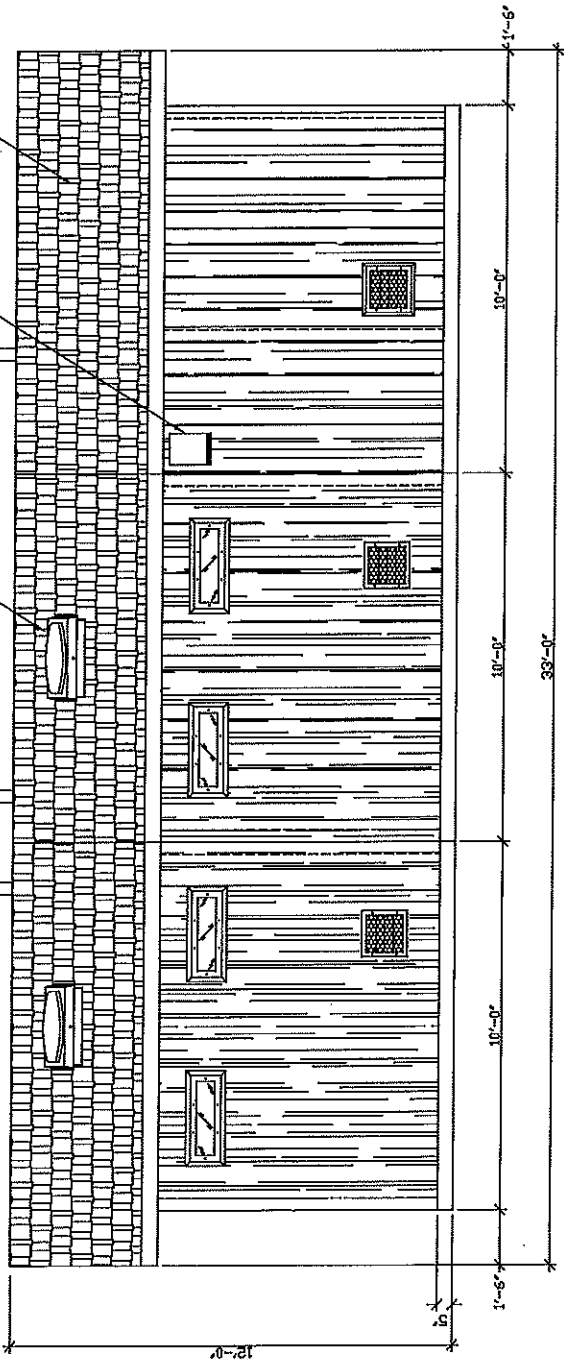
RH SIDE ELEVATION
