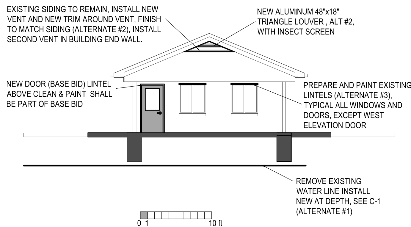
WEST ELEVATION
