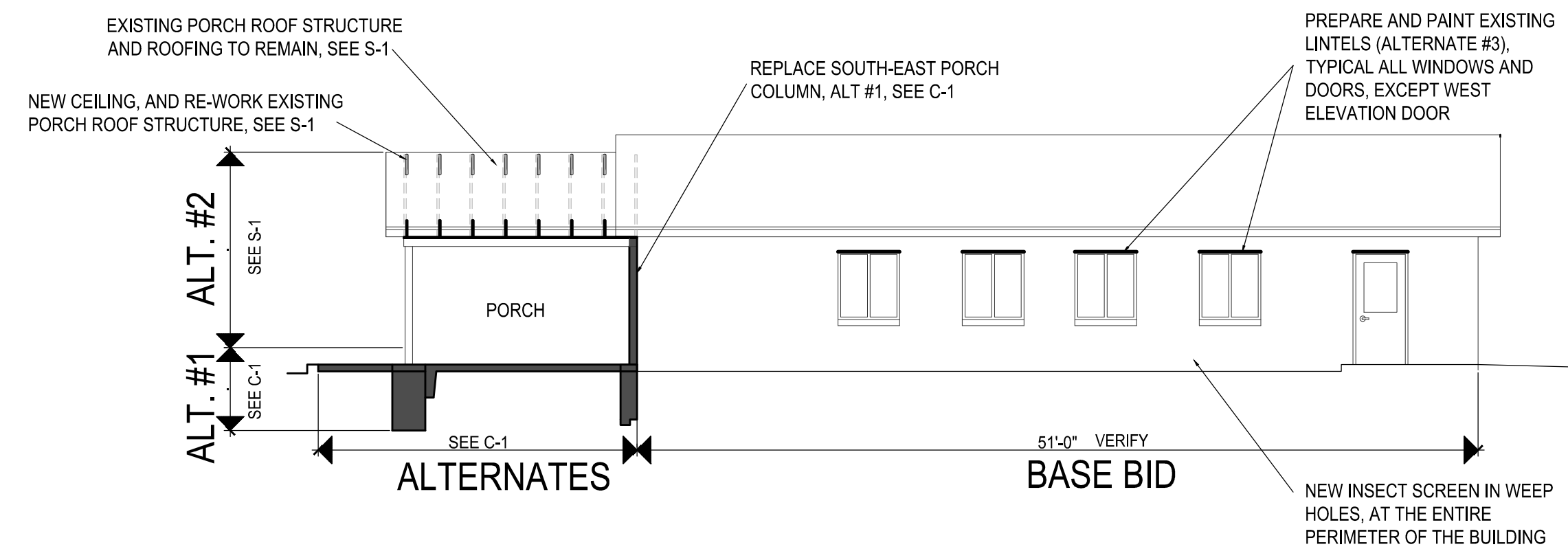
SOUTH ELEVATION
