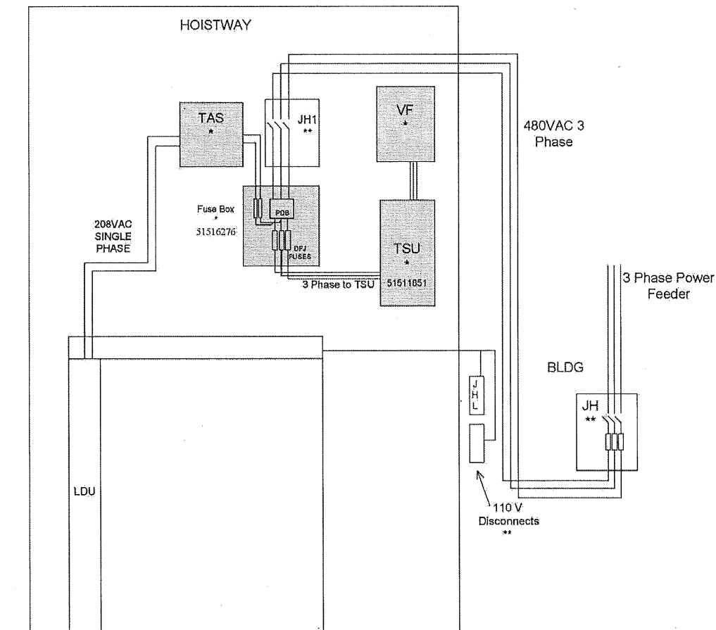
3300 ELECTRICAL SYSTEM LAYOUT – 480 VAC BLDG VOLTAGE
