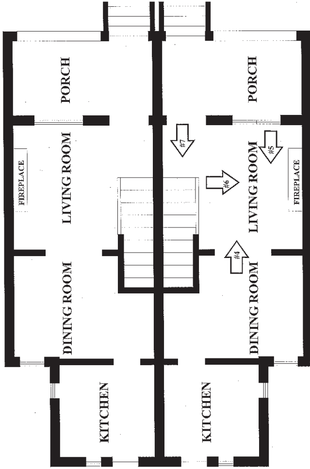
FIRST STORY
