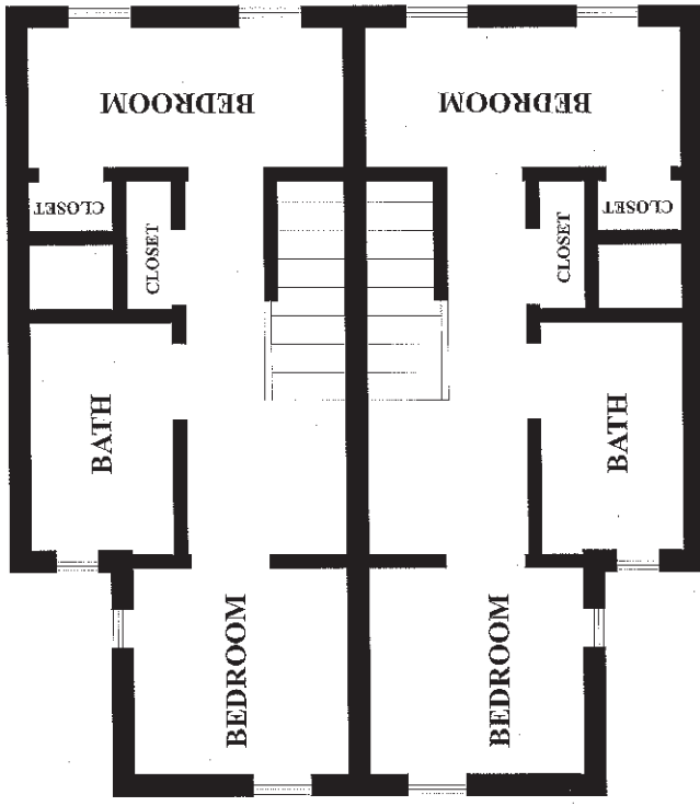
SECOND STORY
